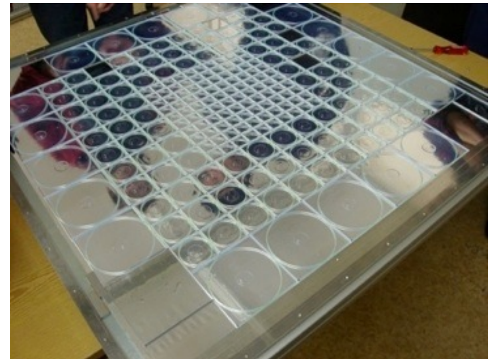
212 scintillator tiles per layer, 38 layers, each channel read out separately
