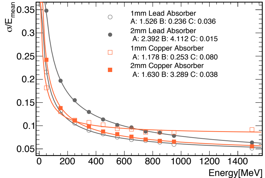
Energy resolution
