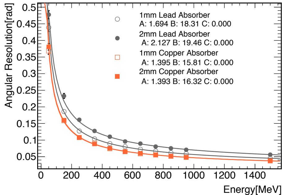
Angular resolution
