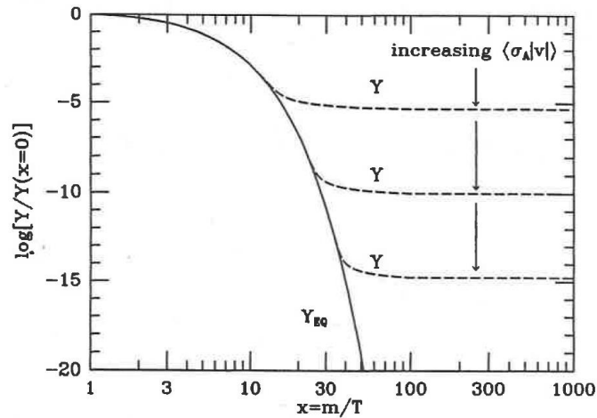
Freeze out of massive particles. Taken from E.Kolb and S. Turner, The early universe
